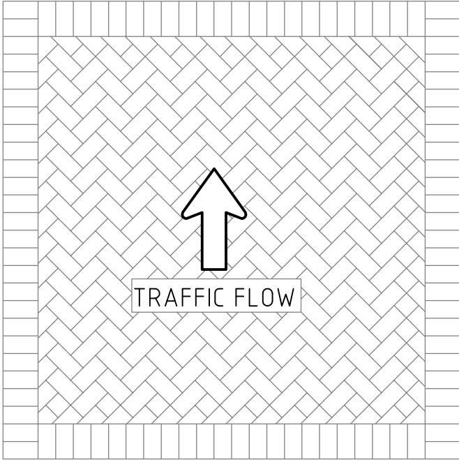
45° HERRINGBONE
