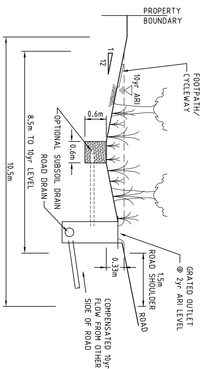
TYPICAL SECTION OF ROADSIDE BIORETENTION BASIN NTS
